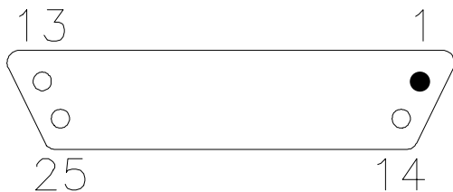
J1 PIN LOCATIONS
